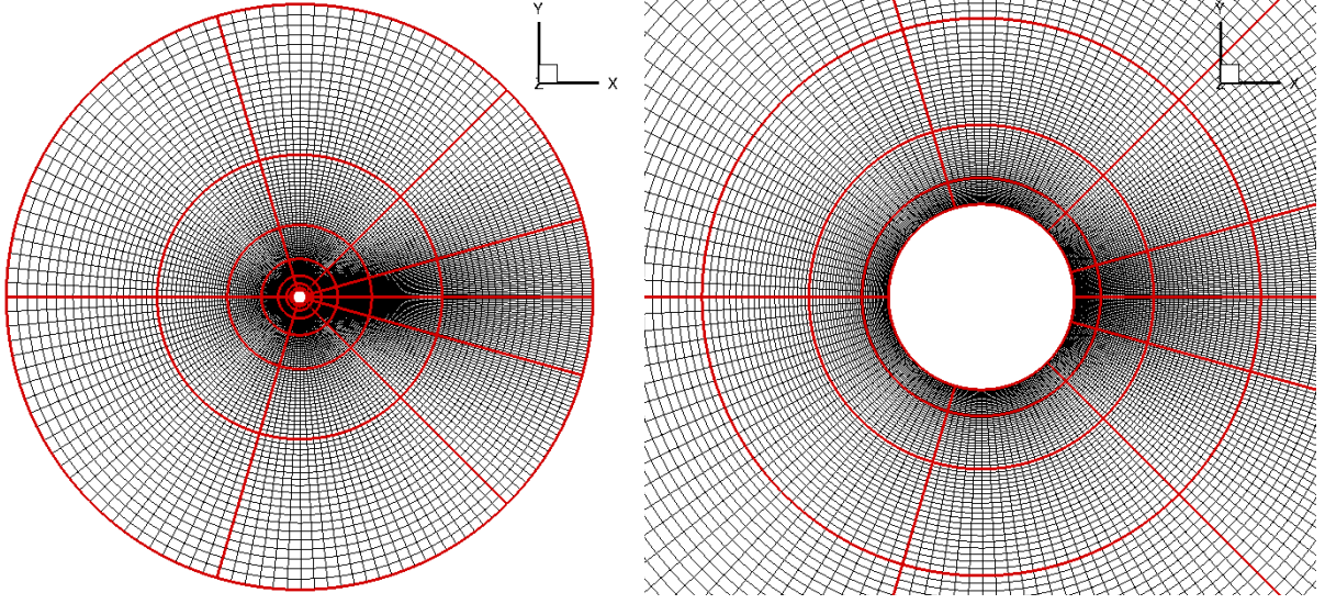
Figure 1: Computational grid with block boundaries highlighted in red
