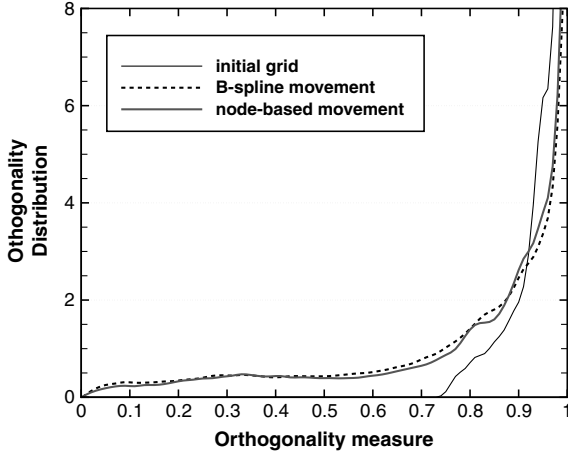
Fig. 6 Orthogonality distribution for the initial flat-plate grid and BWB grids.
