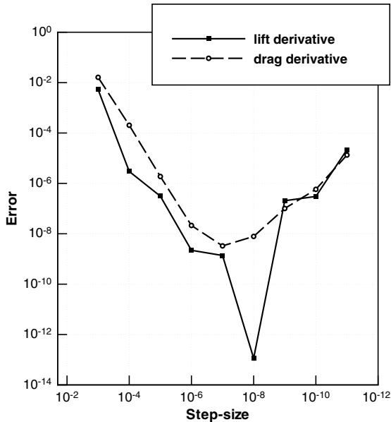
Fig. 10 Relative error between the adjoint-based and second-order-accurate finite difference values of the directional derivative D_\alpha \mathcal{J} .
