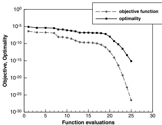
Fig. 11 Convergence history for the inverse design verification.
