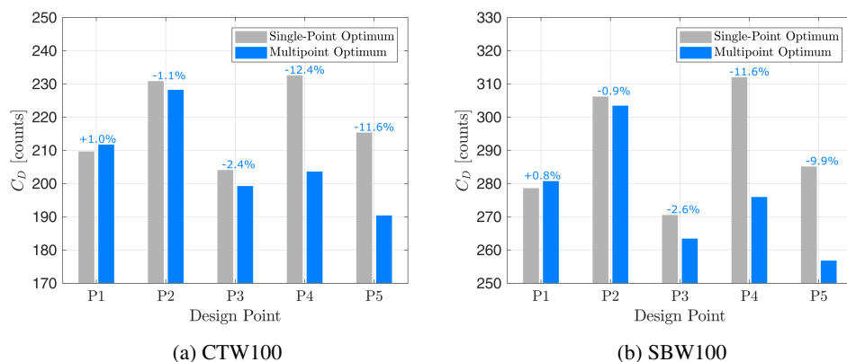
Figure 5: Cruise drag performance at each design point of the five-point operating envelope for each optimised design.
