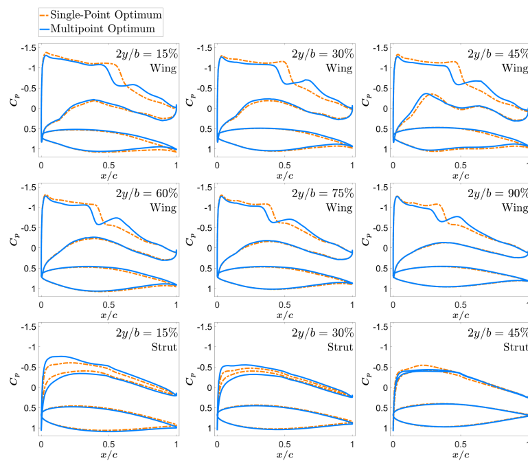
(a) Design point 2: M = 0.78 and C_L = 0.750 (+10% nominal)
