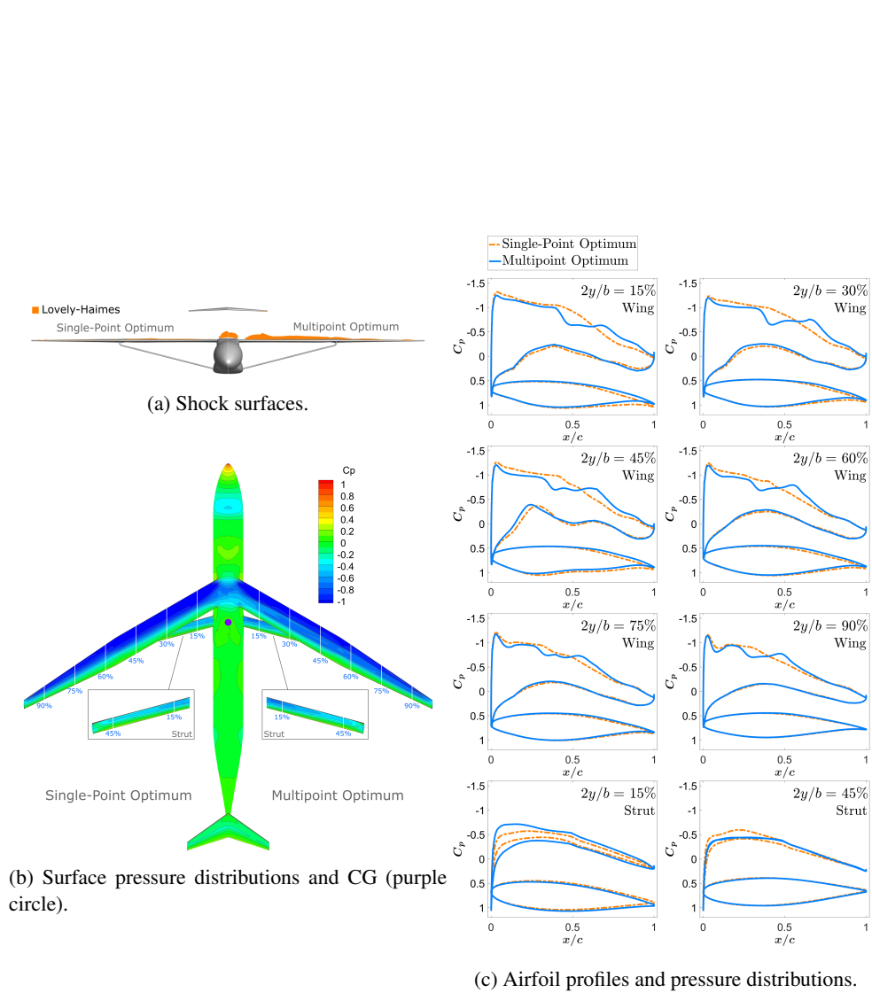
Figure 10: SBW100: Optimised design and flow features calculated on the L0 grid level at the nominal design point ( M = 0.78 and C_L = 0.682 ).
