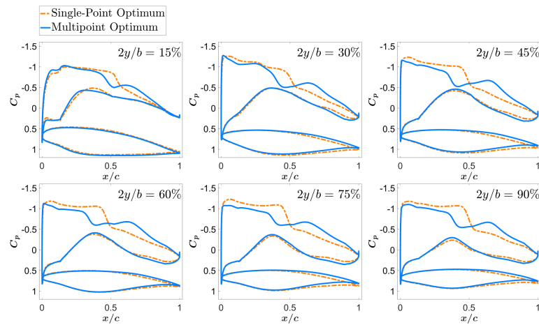
(a) Design point 2: M = 0.78 and C_L = 0.515 (+10% nominal)
