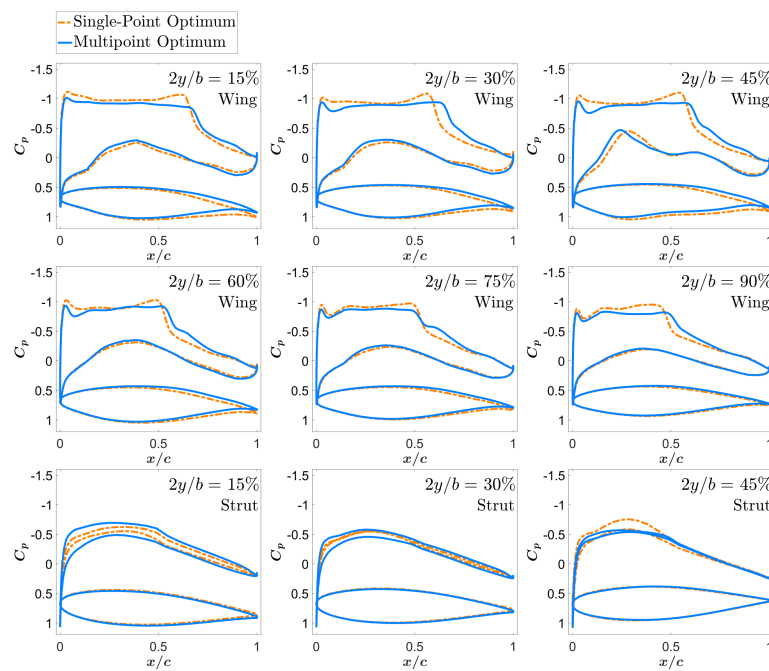
(b) Design point 4: M = 0.81 (nominal +0.03) and C_L = 0.613 (-10% nominal)
