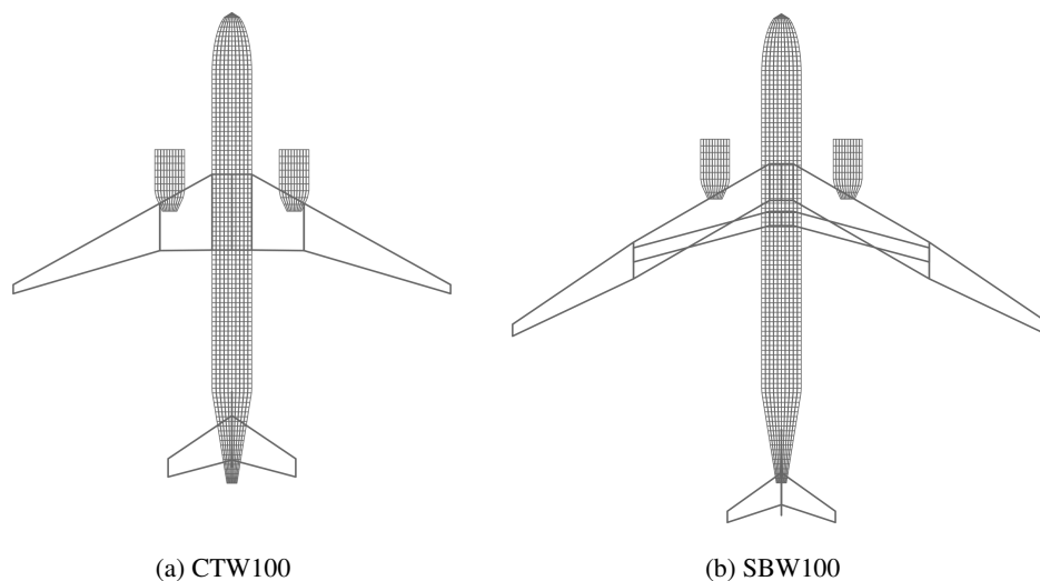
Figure 1: Aircraft concepts developed through conceptual MDO (22) .
