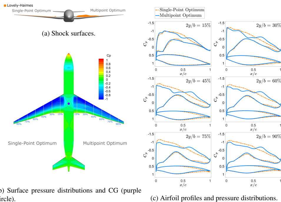
Figure 8: CTW100: Optimised design and flow features computed on the L0 grid level at the nominal design point ( M = 0.78 and C_L = 0.468 ).
