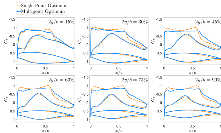
(b) Design point 4: M = 0.81 (nominal +0.03) and C_L = 0.421 (-10% nominal)
