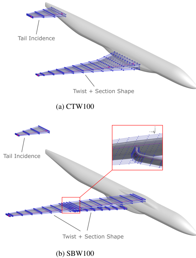
Figure 2: Geometry control systems with FFD volume entities in blue, and axial curve entities in fuschia.
