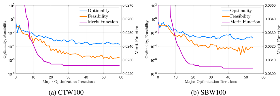
Figure 3: SNOPT optimisation histories.
