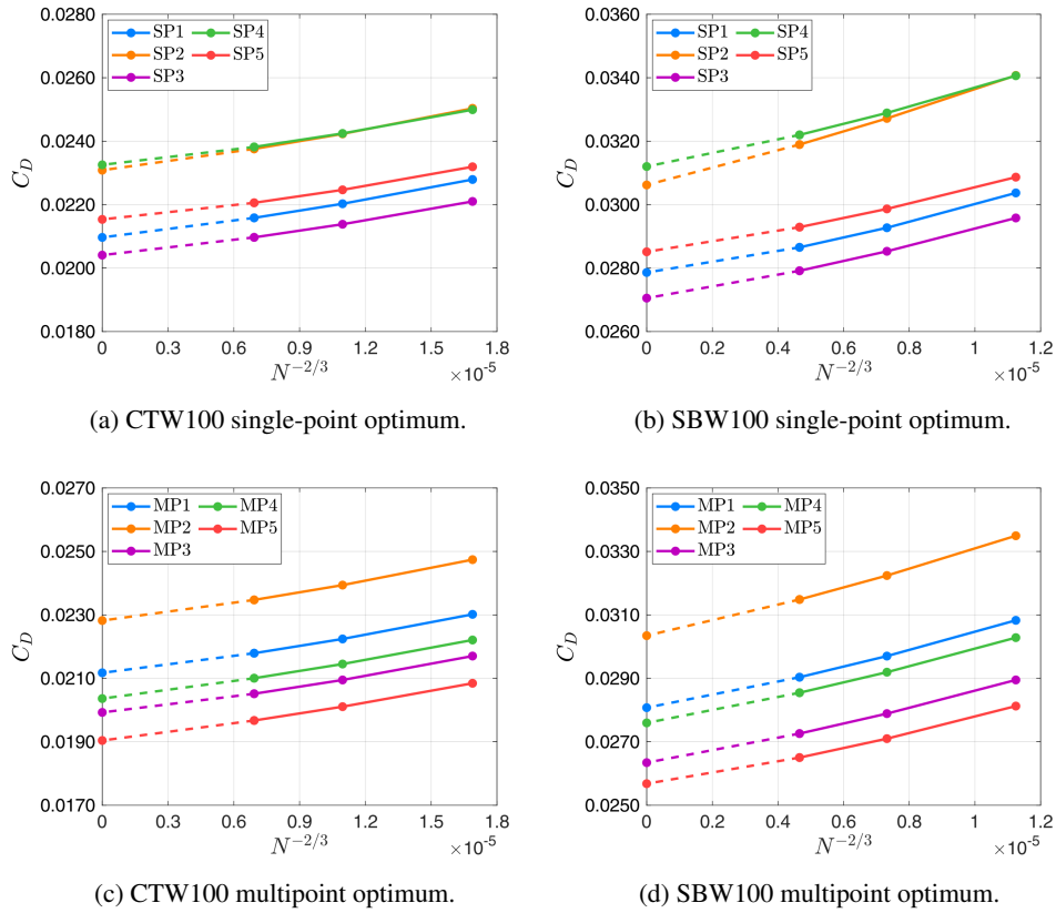
Figure 4: Grid convergence studies for the single-point and multipoint optimised designs at constant lift, evaluated at each of the five design points. Drag coefficients at N^{-2/3} = 0 are obtained from Richardson extrapolation.
